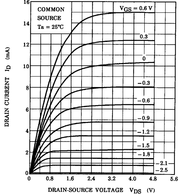
ID - VDS (LOW VOLTAGE REGION)
