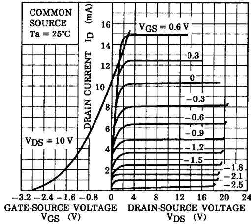
STATIC CHARACTERISTICS
